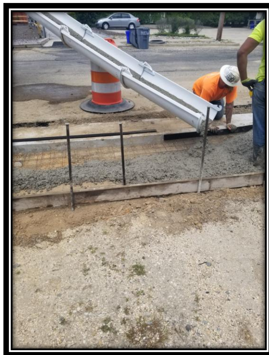
Figure: 3 – Installation of concrete driveway apron on West Atlantic Avenue along the westbound lane between South Main Street and South Boyd Street
